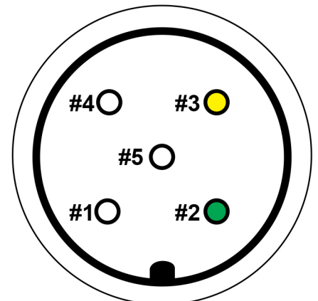
Male M12 5-pin Connector (End View)
